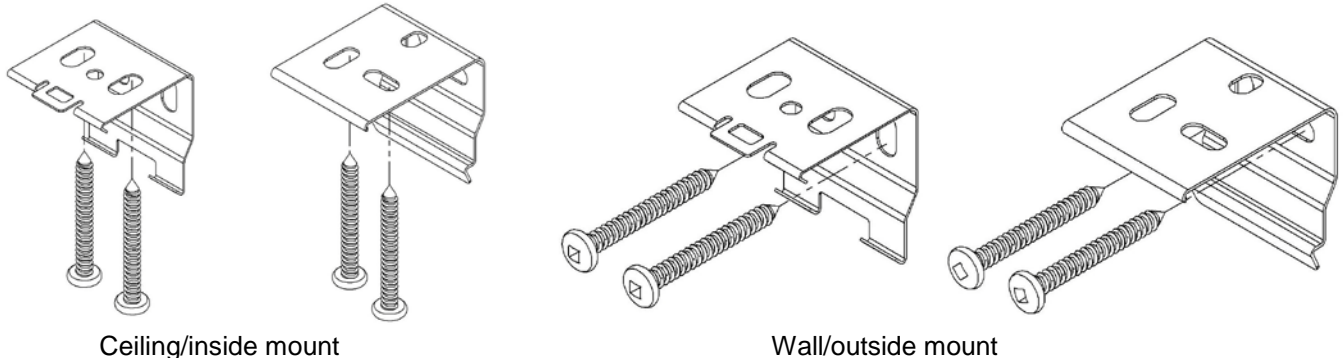
Ceiling/inside mount
