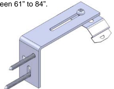
Fig. 4 Lateral mount
